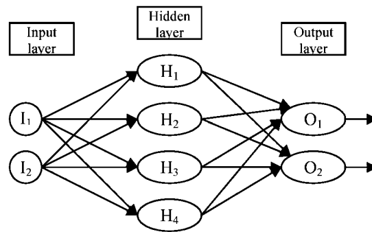
Fig. 4. ANN structure.
