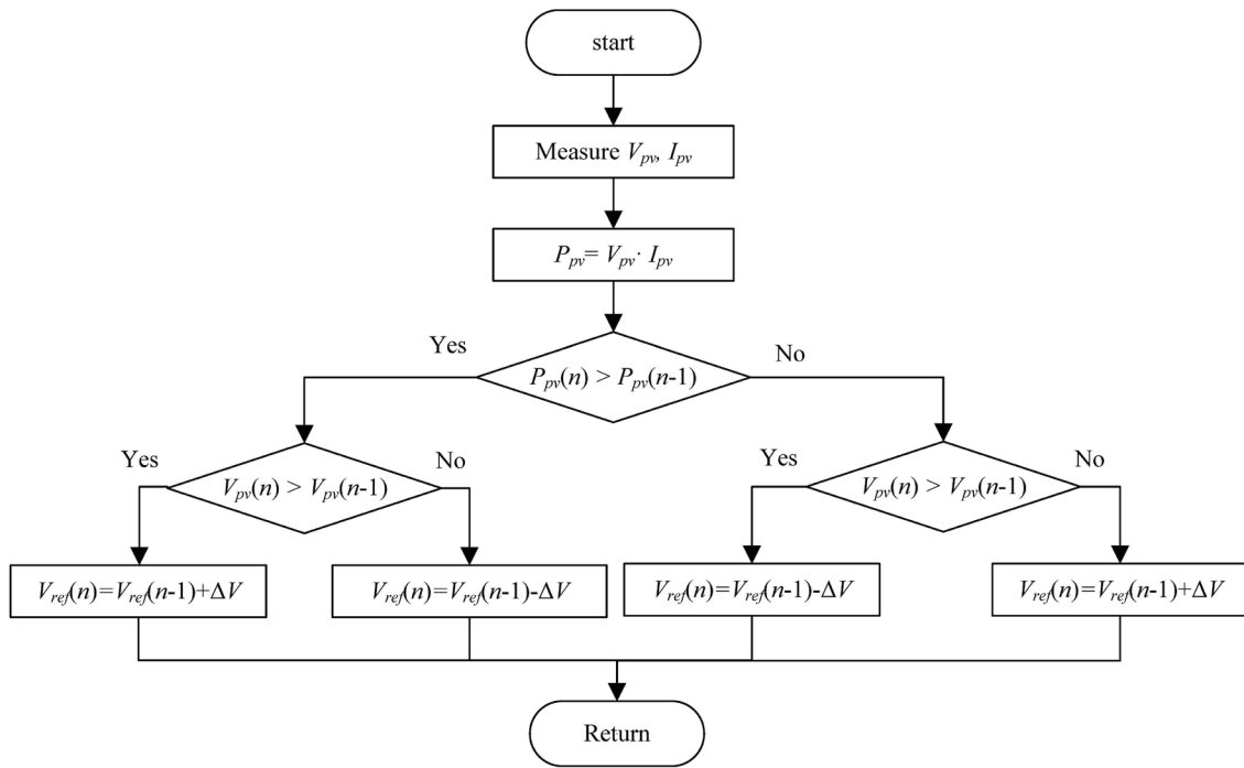
Fig. 2. P&O algorithm flowchart.
