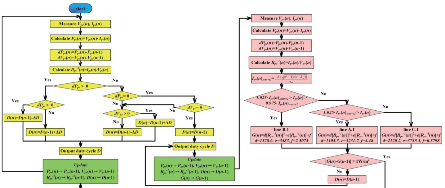
Fig. 6. (Color online) Flowchart of the proposed algorithm.
