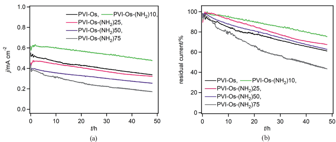
Fig. 3. (Color online) (a) Chronoamperograms of LOx-hydrogel-modified MgOC electrodes using PVI-Os-(NH 2 ) at various quaternization ratios. LOx, PVI-Os, and PEGDGE in a ratio of 20:70:10 were deposited on the MgOC electrode at 600 \mu\text{g cm}^{-2} . Measurement conditions: 0.6 V, pH 7.0, phosphate buffer solution (0.1 M) containing lactate (0.1 M), and 25 °C. (b) Residual current vs time.
