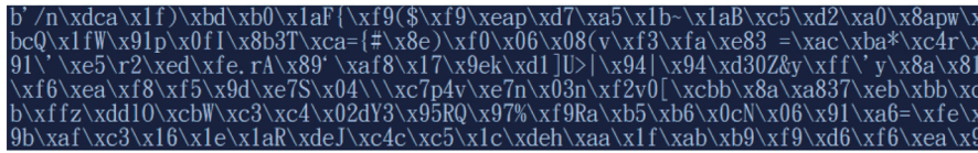
Fig. 12. Received data.
